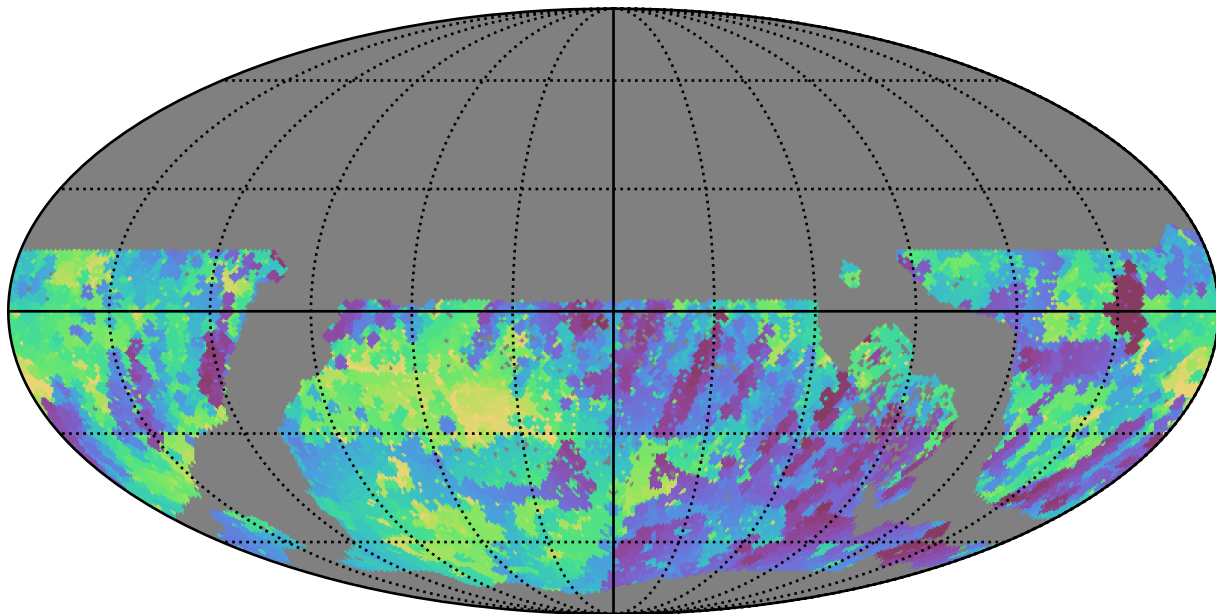
too_5_1v3.4_10yrs WFD r band: Min skyBrightness
