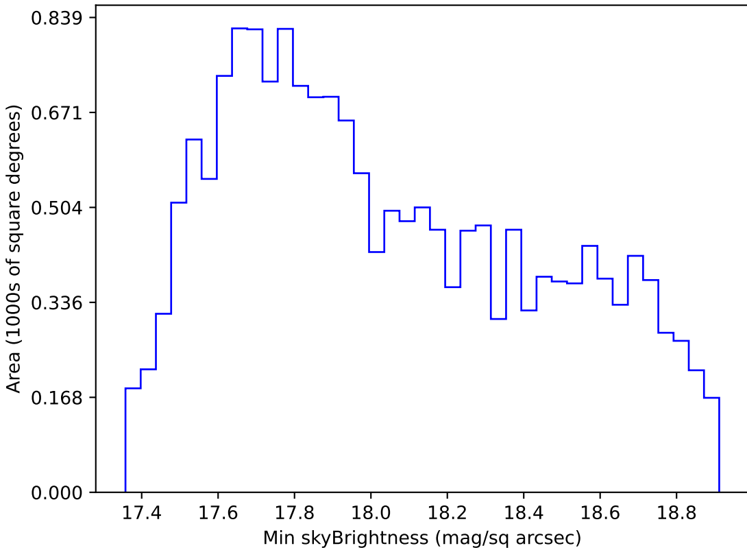
too_5_1v3.4_10yrs WFD i band: Min skyBrightness
