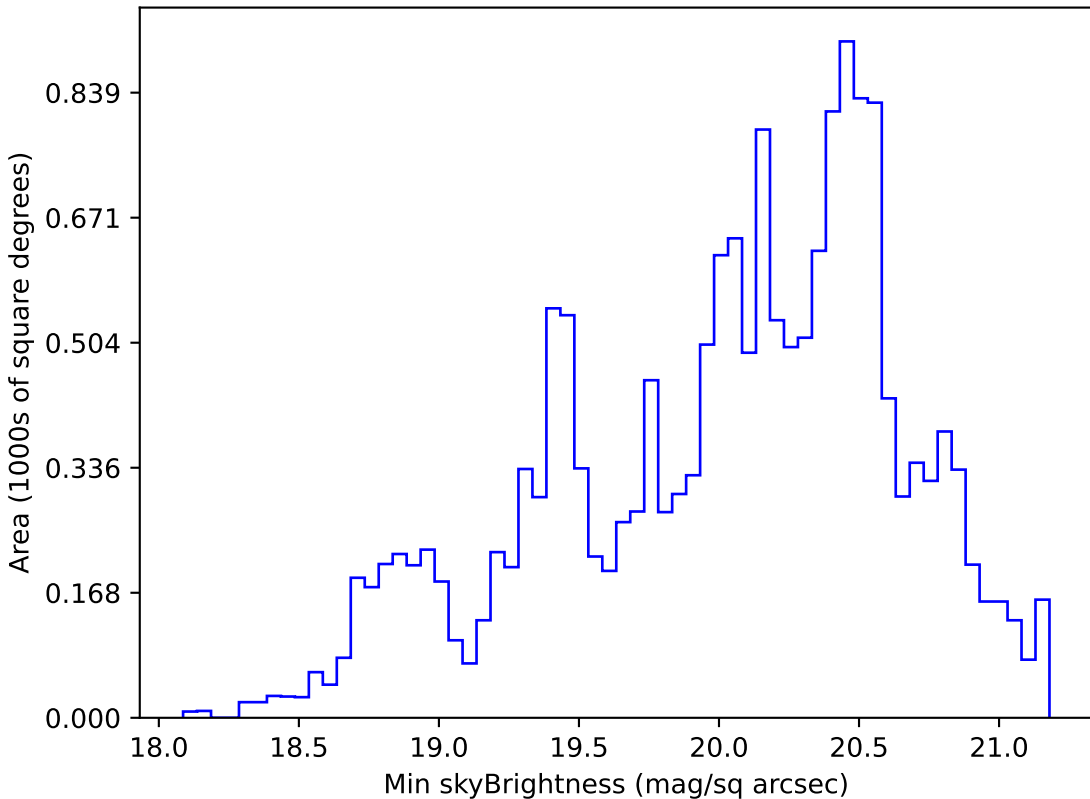
too_5_1v3.4_10yrs WFD g band: Min skyBrightness
