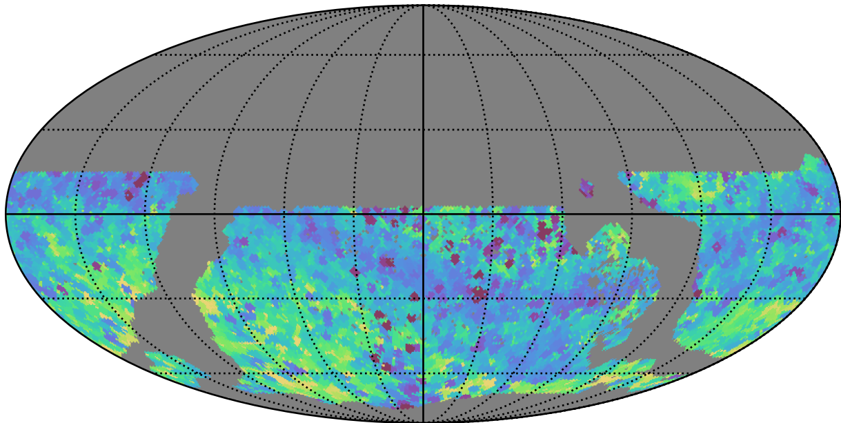
too_5_1v3.4_10yrs WFD all bands: Min skyBrightness
