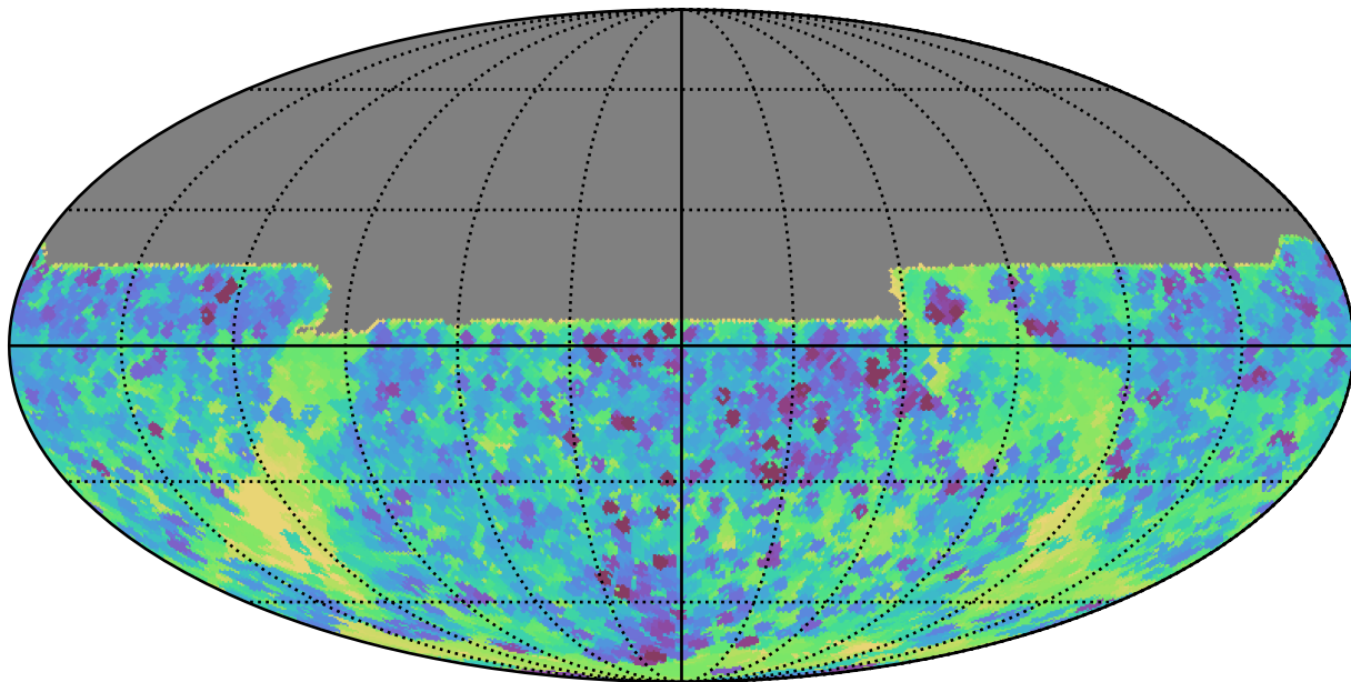
too_5_1v3.4_10yrs All sky y band: Min skyBrightness
