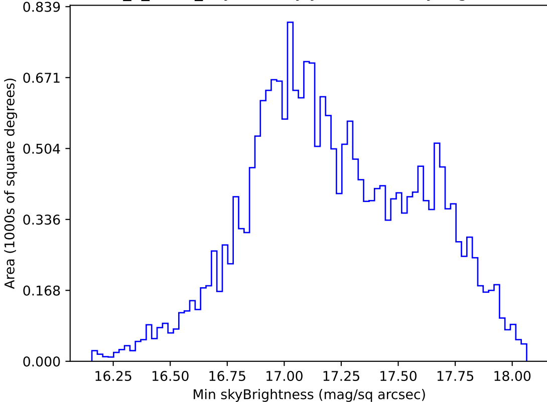
too_5_1v3.4_10yrs All sky y band: Min skyBrightness
