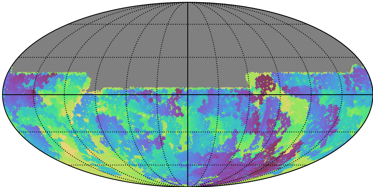
too_5_1v3.4_10yrs All sky u band: Min skyBrightness
