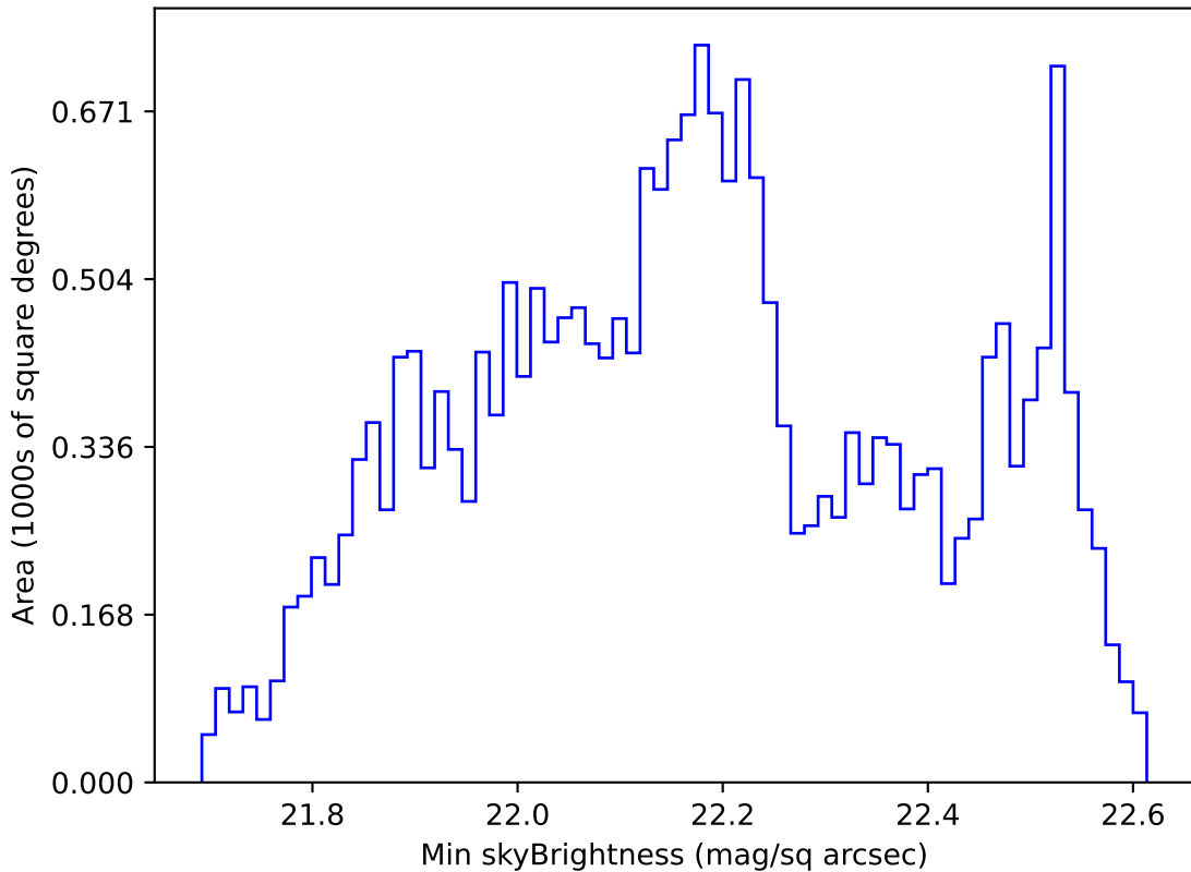
too_5_1v3.4_10yrs All sky u band: Min skyBrightness
