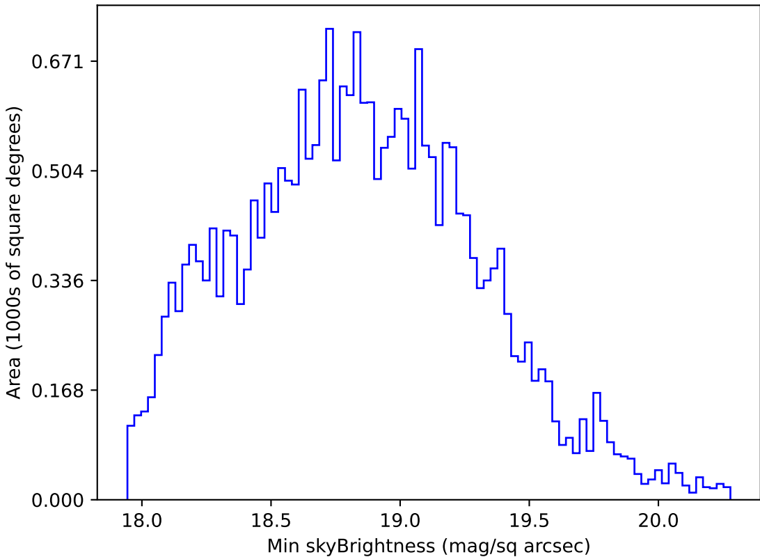
too_5_1v3.4_10yrs All sky r band: Min skyBrightness
