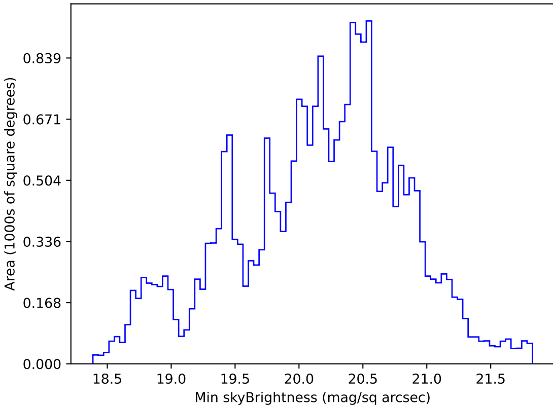
too_5_1v3.4_10yrs All sky g band: Min skyBrightness
