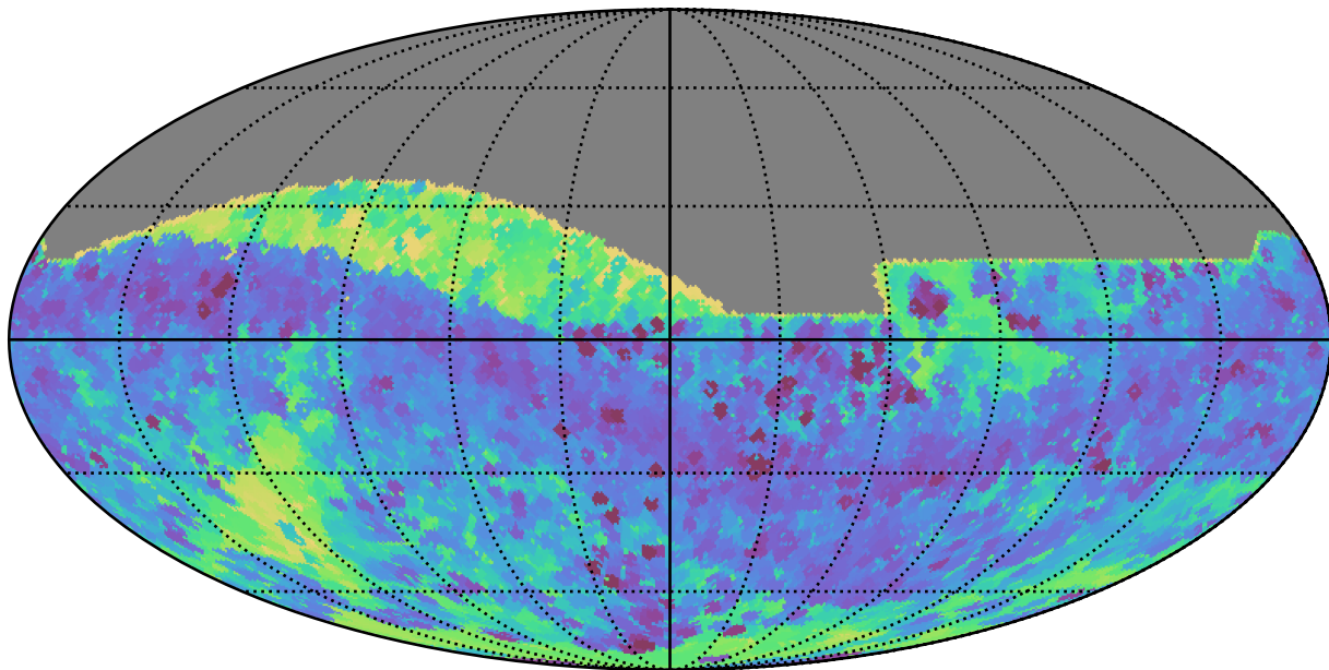
too_5_1v3.4_10yrs All sky all bands: Min skyBrightness
