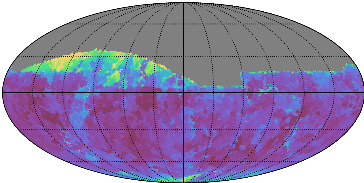
too_5_1v3.4_10yrs Yr 1 z band: Min seeingGeom
