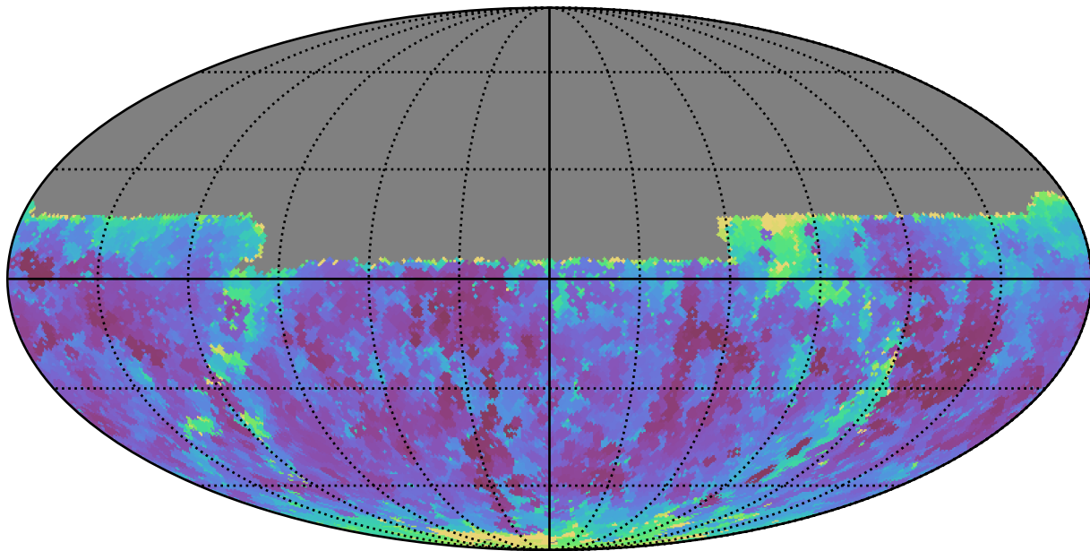
too_5_1v3.4_10yrs Yr 1 y band: Min seeingGeom
