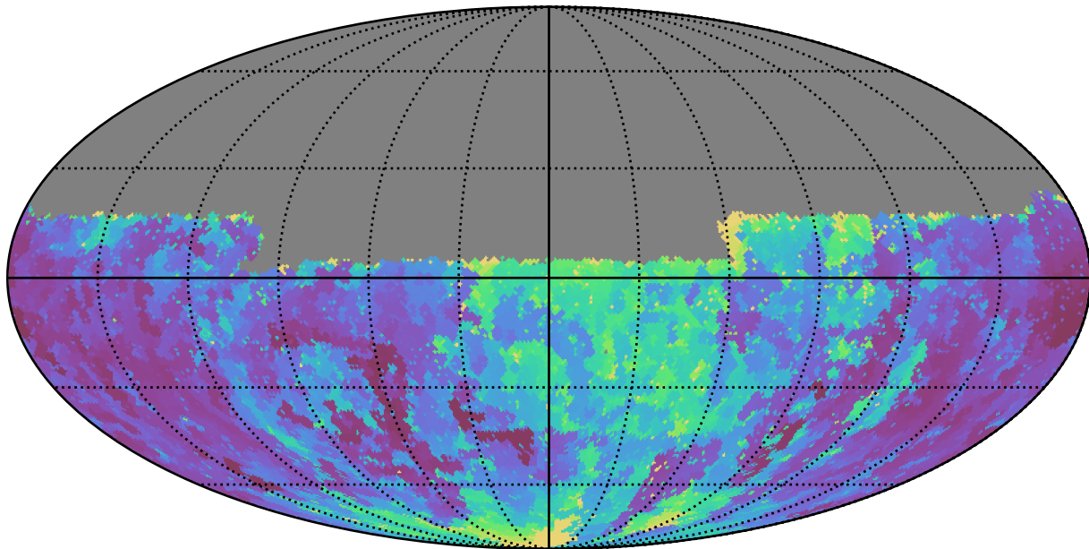
too_5_1v3.4_10yrs Yr 1 u band: Min seeingGeom
