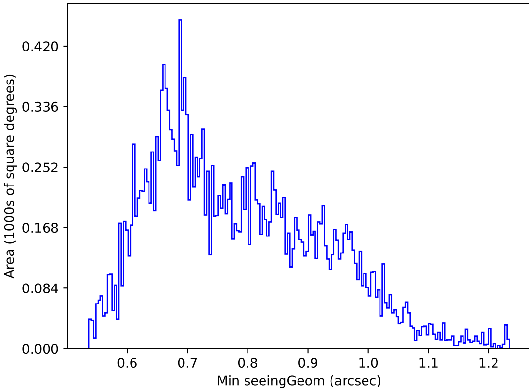
too_5_1v3.4_10yrs Yr 1 u band: Min seeingGeom
