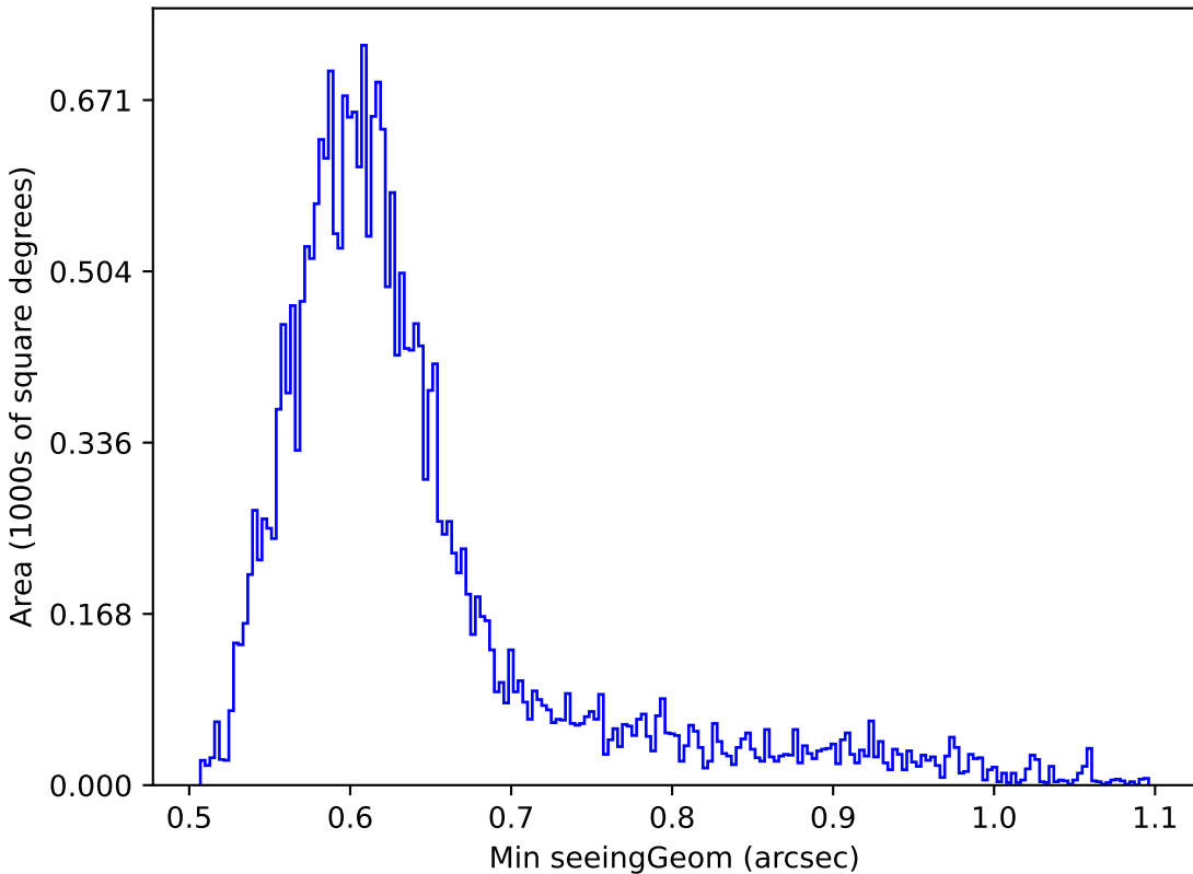
too_5_1v3.4_10yrs Yr 1 r band: Min seeingGeom
