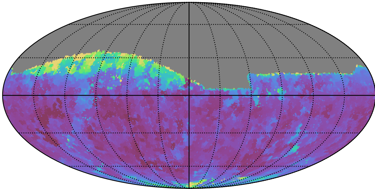
too_5_1v3.4_10yrs Yr 1 i band: Min seeingGeom
