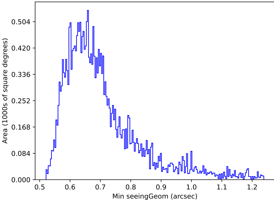
too_5_1v3.4_10yrs Yr 1 g band: Min seeingGeom
