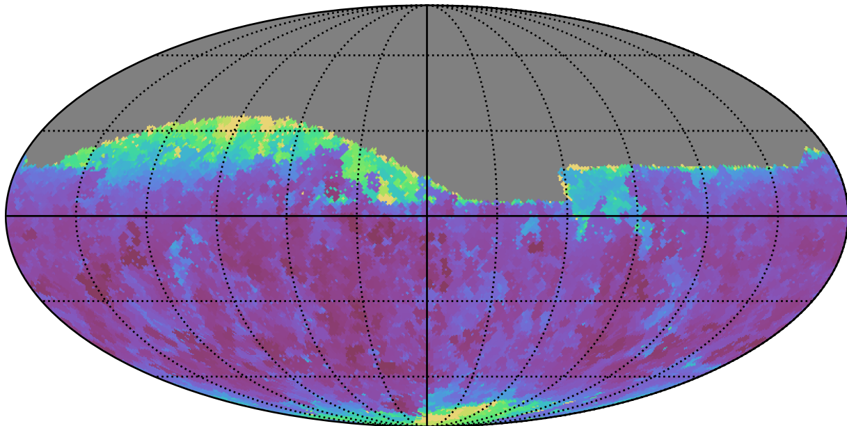
too_5_1v3.4_10yrs Yr 1 r band: Min seeingEff
