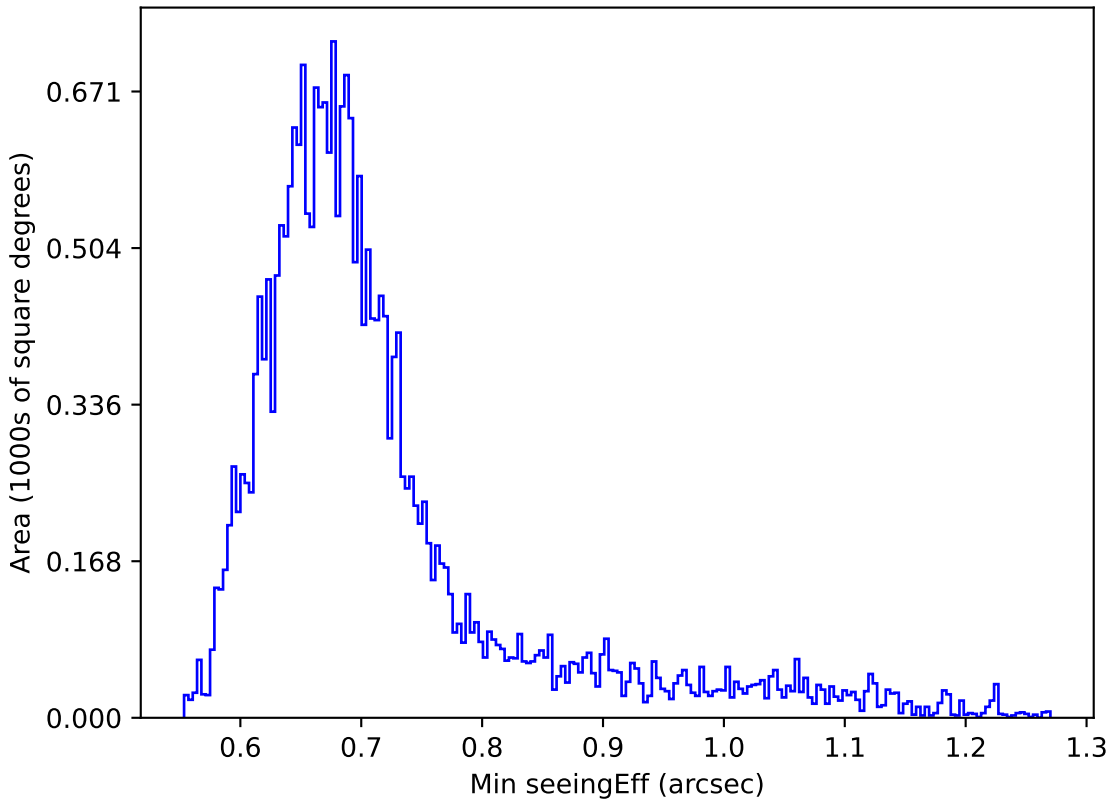
too_5_1v3.4_10yrs Yr 1 r band: Min seeingEff
