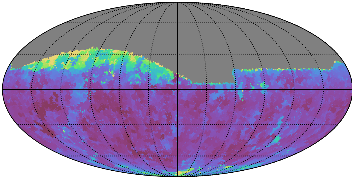
too_5_1v3.4_10yrs Yr 1 i band: Min seeingEff
