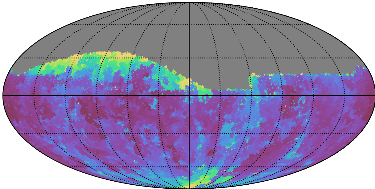
too_5_1v3.4_10yrs Yr 1 g band: Min seeingEff
