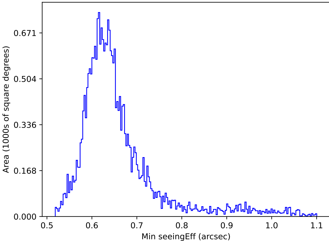
too_5_1v3.4_10yrs Yr 1 all bands: Min seeingEff
