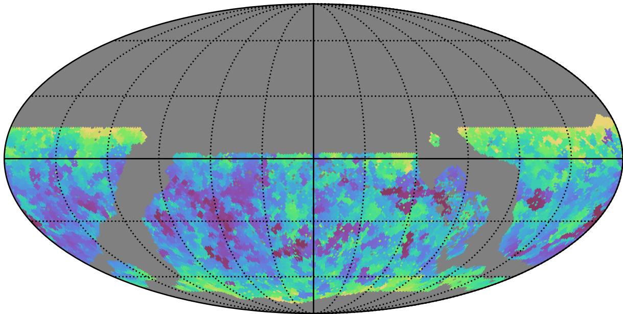
too_5_1v3.4_10yrs WFD z band: Min seeingEff
