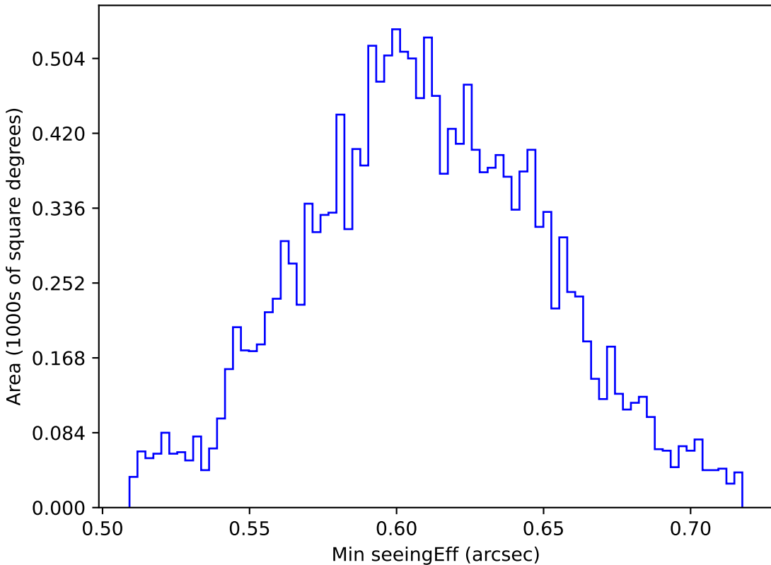
too_5_1v3.4_10yrs WFD z band: Min seeingEff
