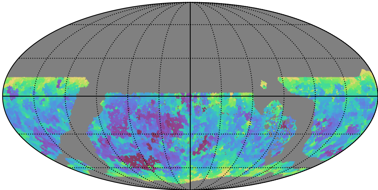
too_5_1v3.4_10yrs WFD y band: Min seeingEff
