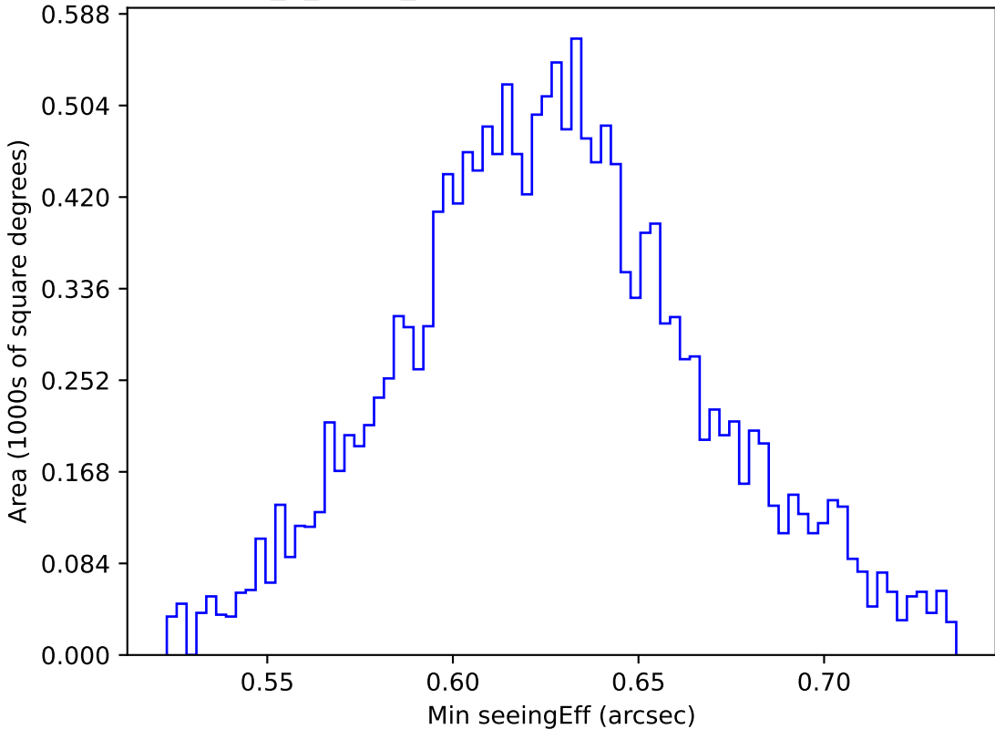
too_5_1v3.4_10yrs WFD y band: Min seeingEff
