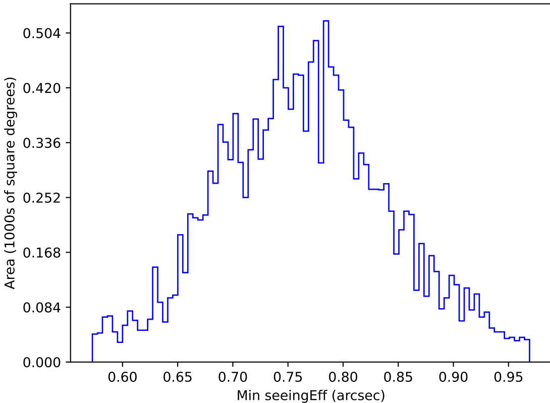
too_5_1v3.4_10yrs WFD u band: Min seeingEff
