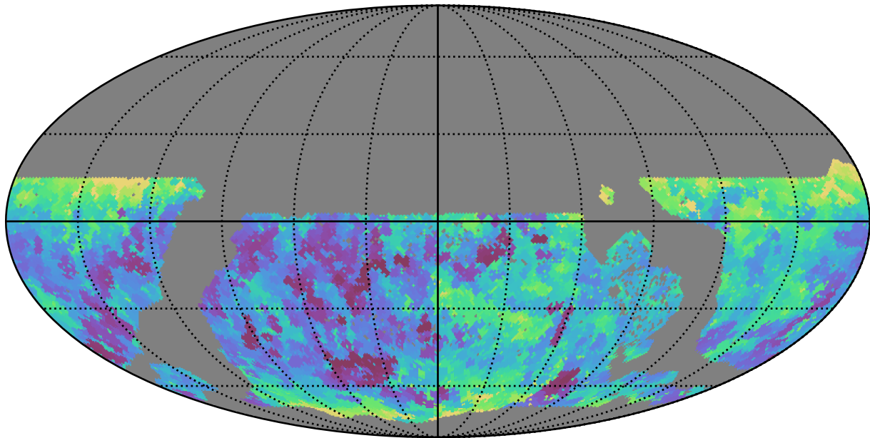
too_5_1v3.4_10yrs WFD i band: Min seeingEff
