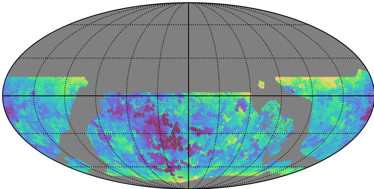
too_5_1v3.4_10yrs WFD g band: Min seeingEff
