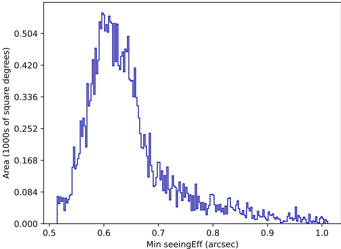
too_5_1v3.4_10yrs All sky z band: Min seeingEff
