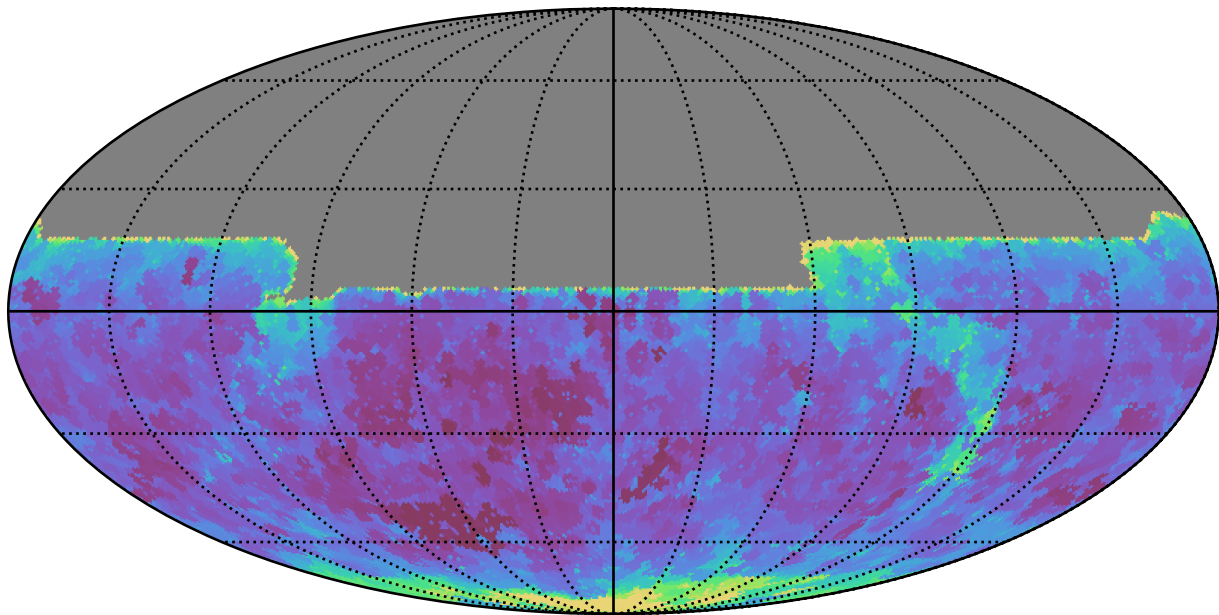
too_5_1v3.4_10yrs All sky y band: Min seeingEff
