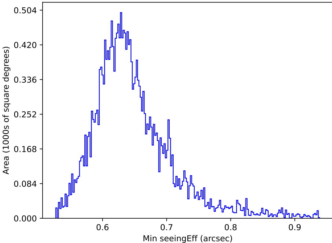
too_5_1v3.4_10yrs All sky y band: Min seeingEff
