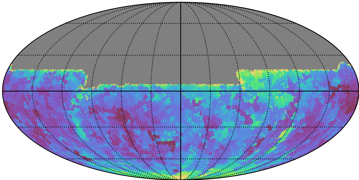
too_5_1v3.4_10yrs All sky u band: Min seeingEff
