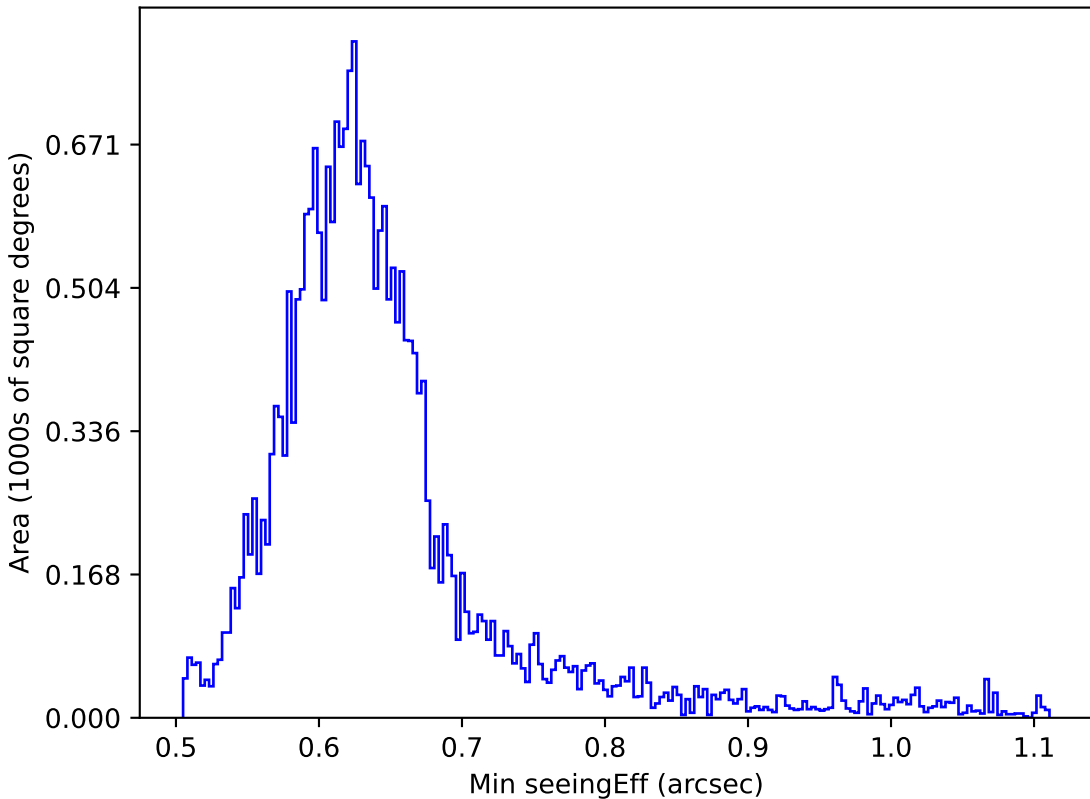
too_5_1v3.4_10yrs All sky r band: Min seeingEff
