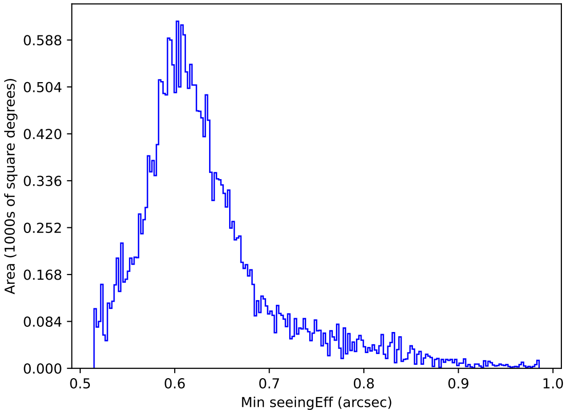
too_5_1v3.4_10yrs All sky i band: Min seeingEff
