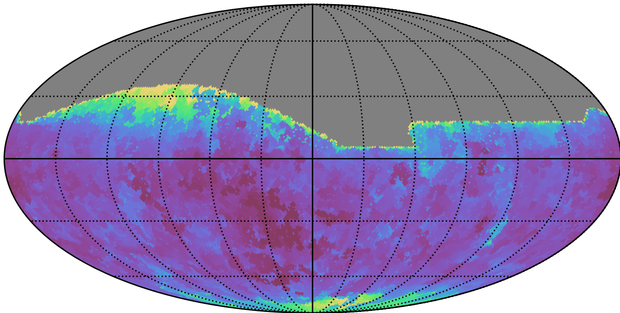
too_5_1v3.4_10yrs All sky g band: Min seeingEff
