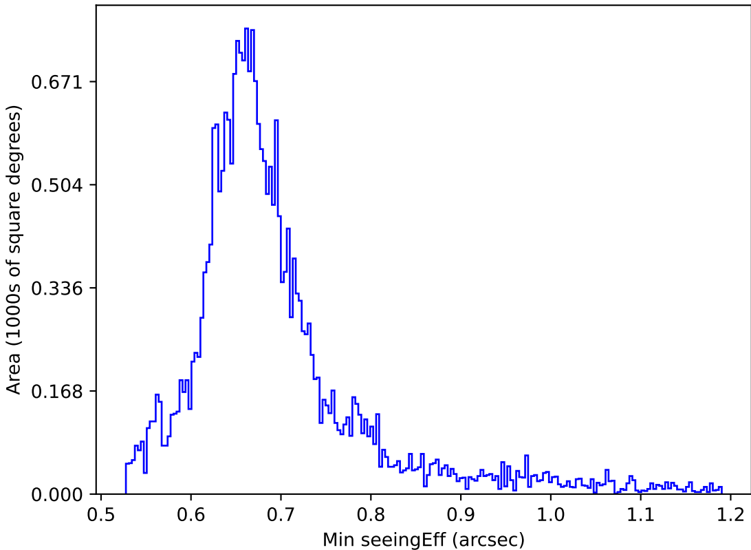
too_5_1v3.4_10yrs All sky g band: Min seeingEff
