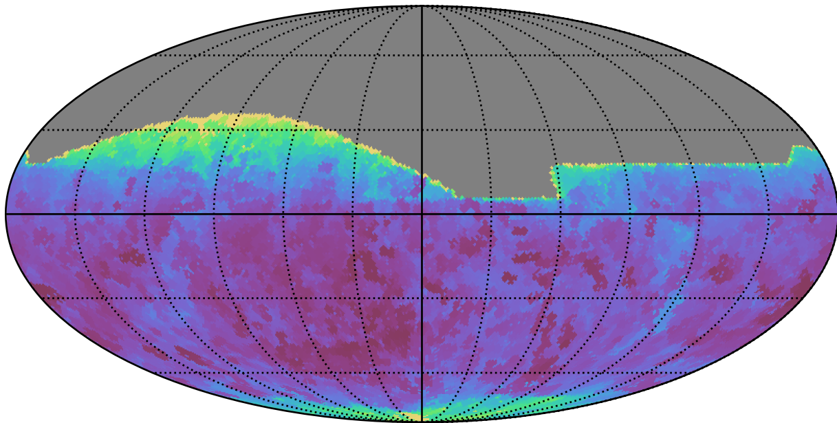
too_5_1v3.4_10yrs All sky all bands: Min seeingEff
