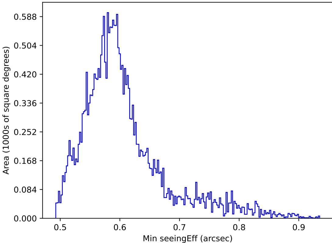
too_5_1v3.4_10yrs All sky all bands: Min seeingEff
