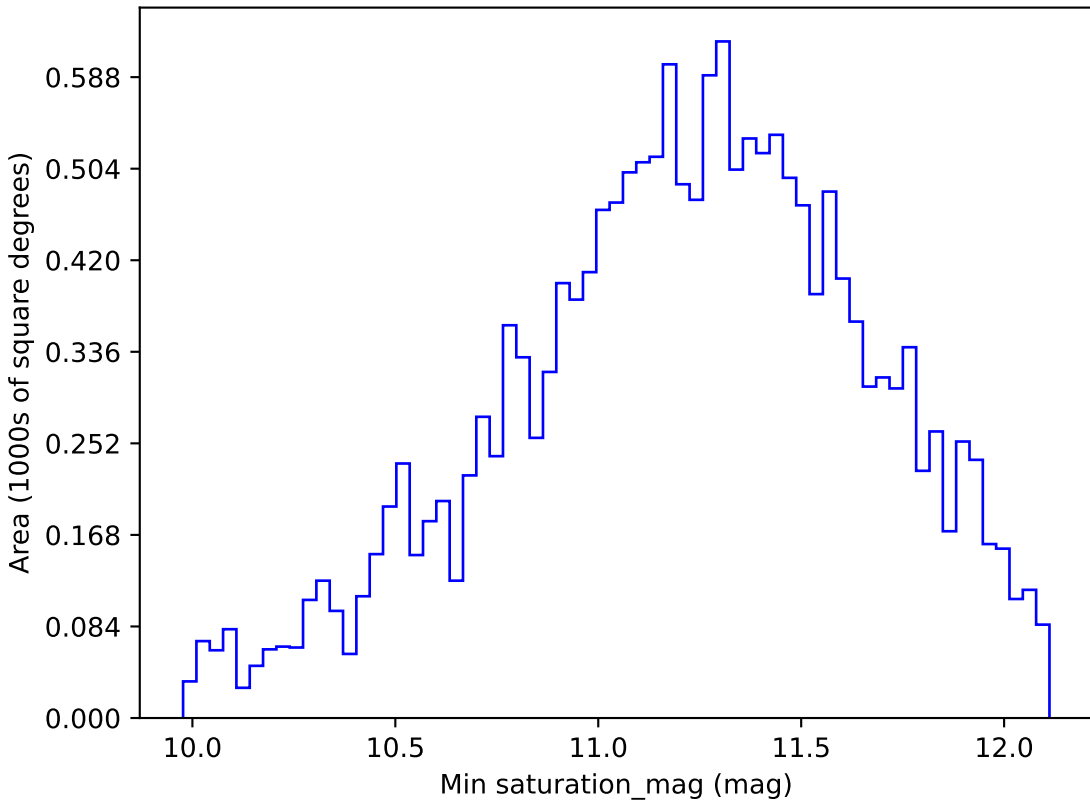
too_5_1v3.4_10yrs WFD y band: Min saturation_mag
