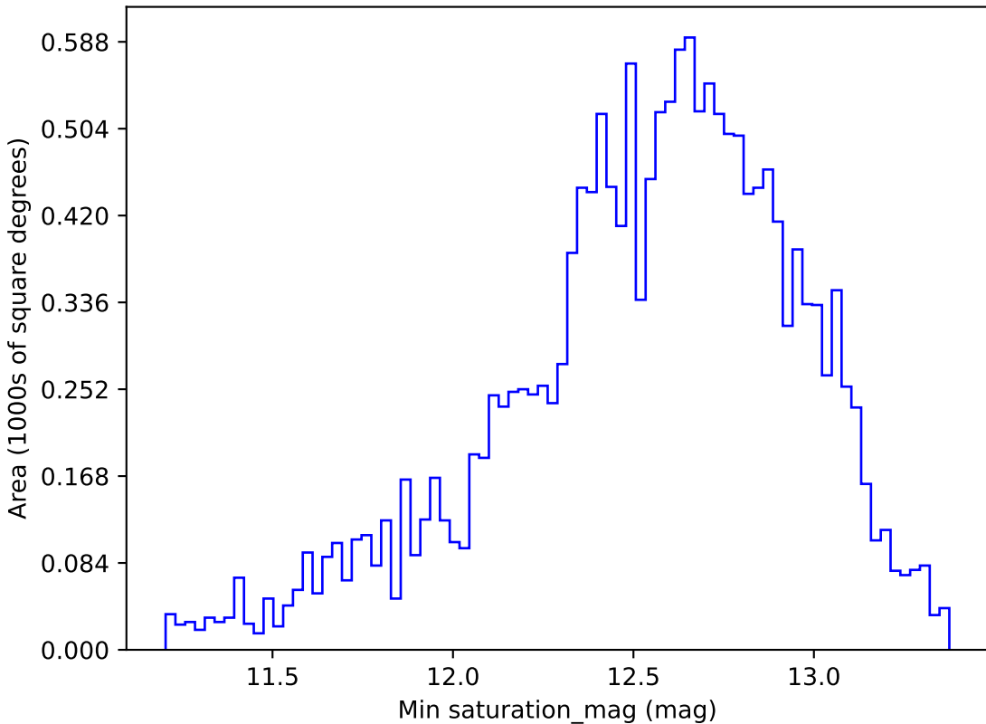
too_5_1v3.4_10yrs WFD r band: Min saturation_mag
