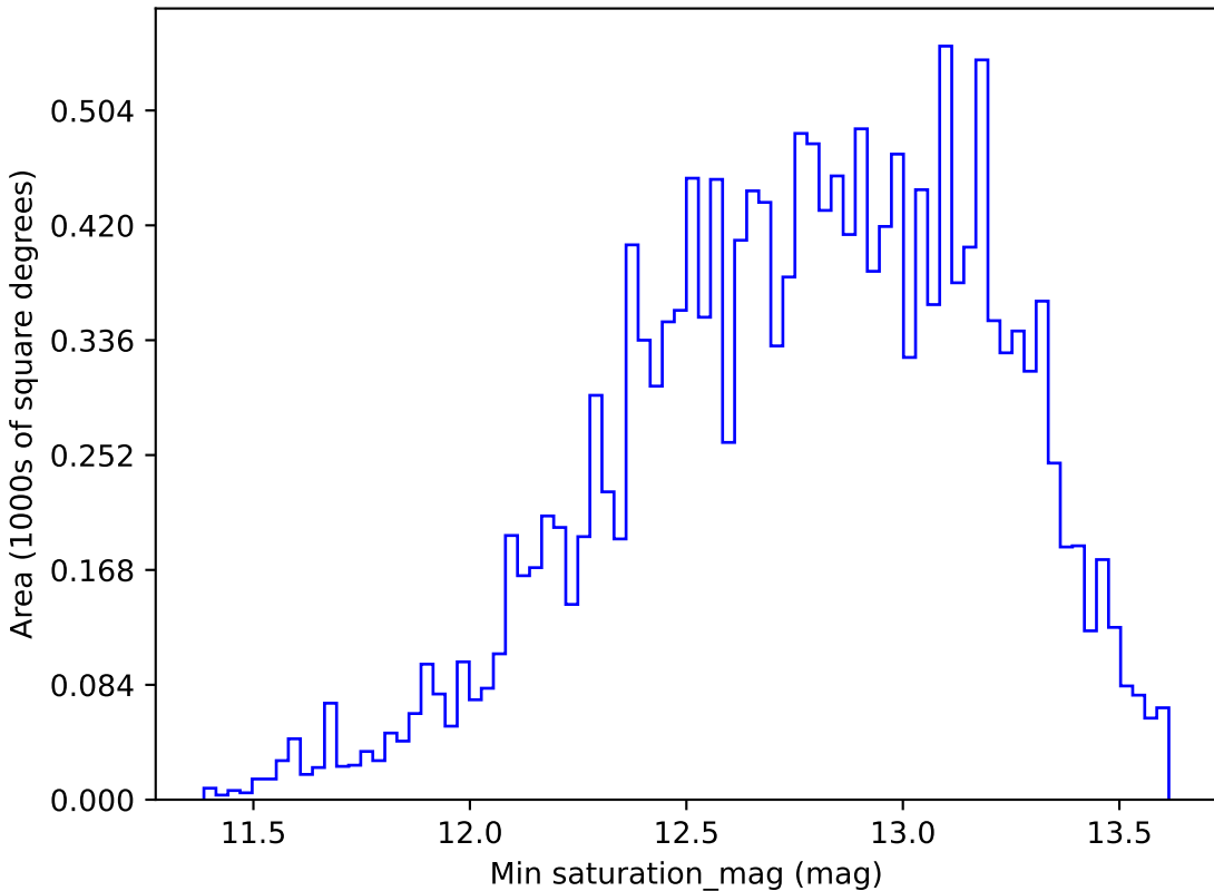
too_5_1v3.4_10yrs WFD g band: Min saturation_mag
