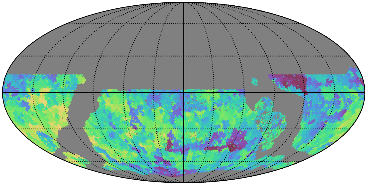
too_5_1v3.4_10yrs WFD all bands: Min saturation_mag
