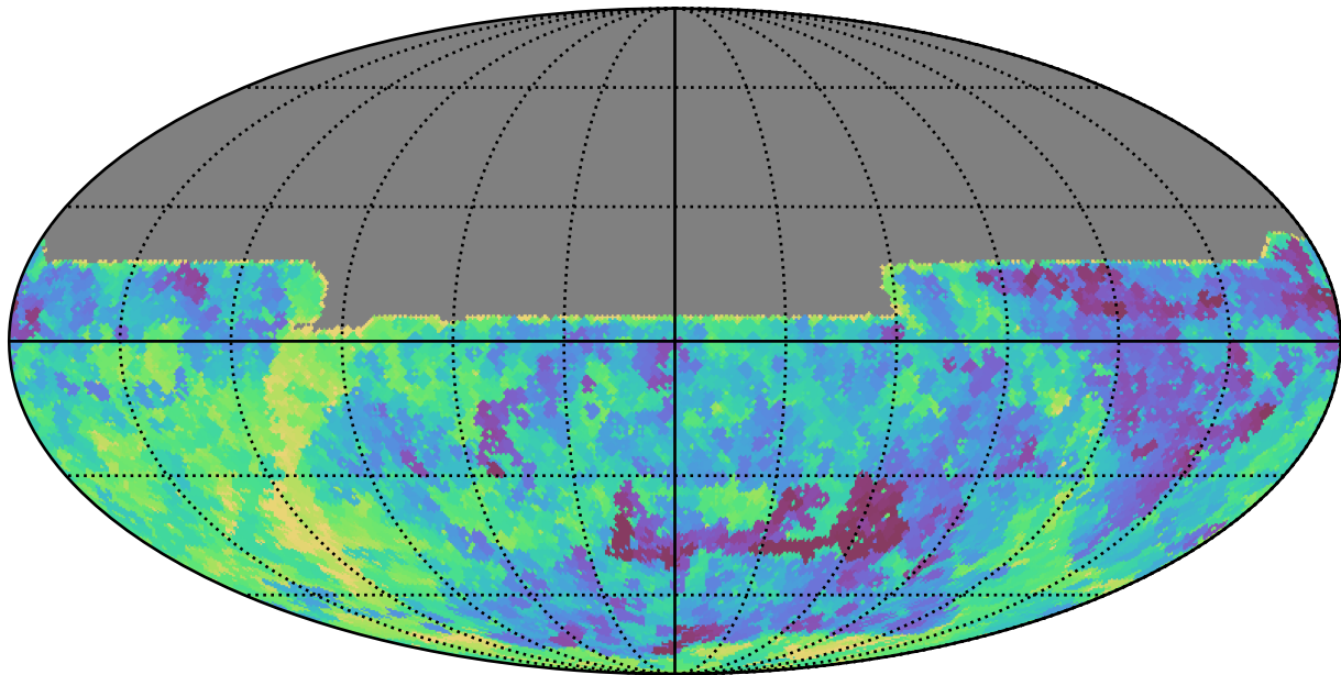
too_5_1v3.4_10yrs All sky y band: Min saturation_mag
