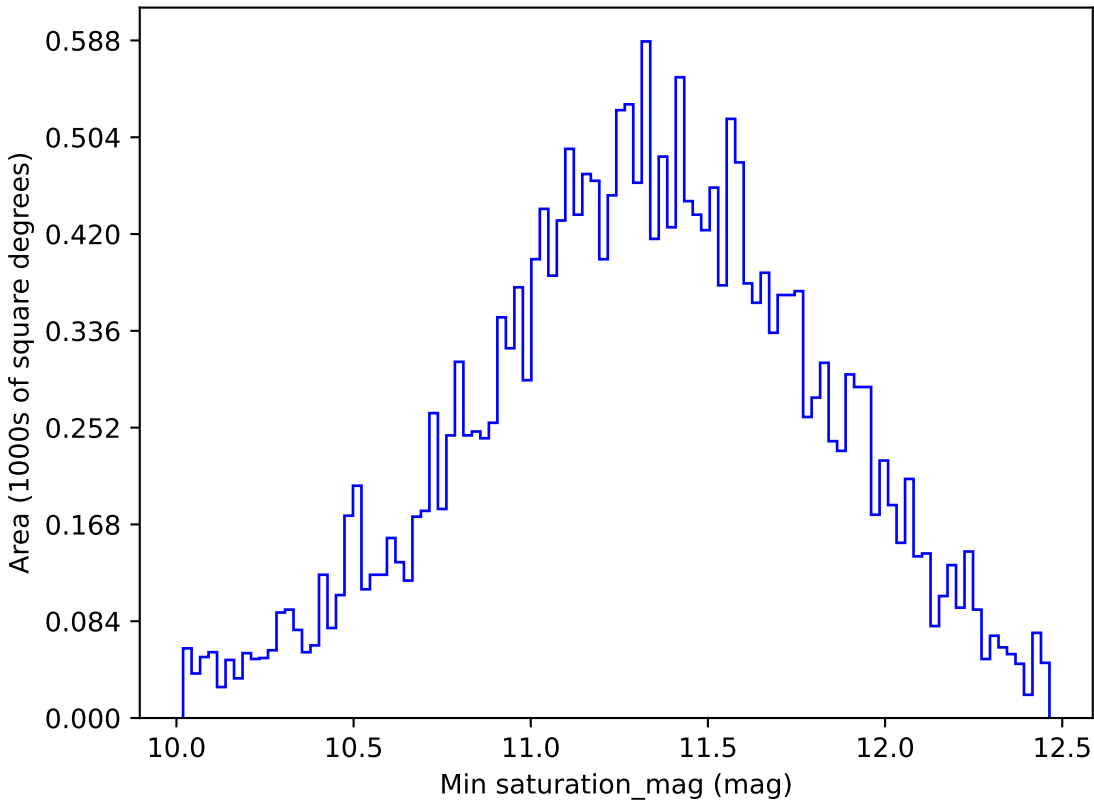
too_5_1v3.4_10yrs All sky y band: Min saturation_mag
