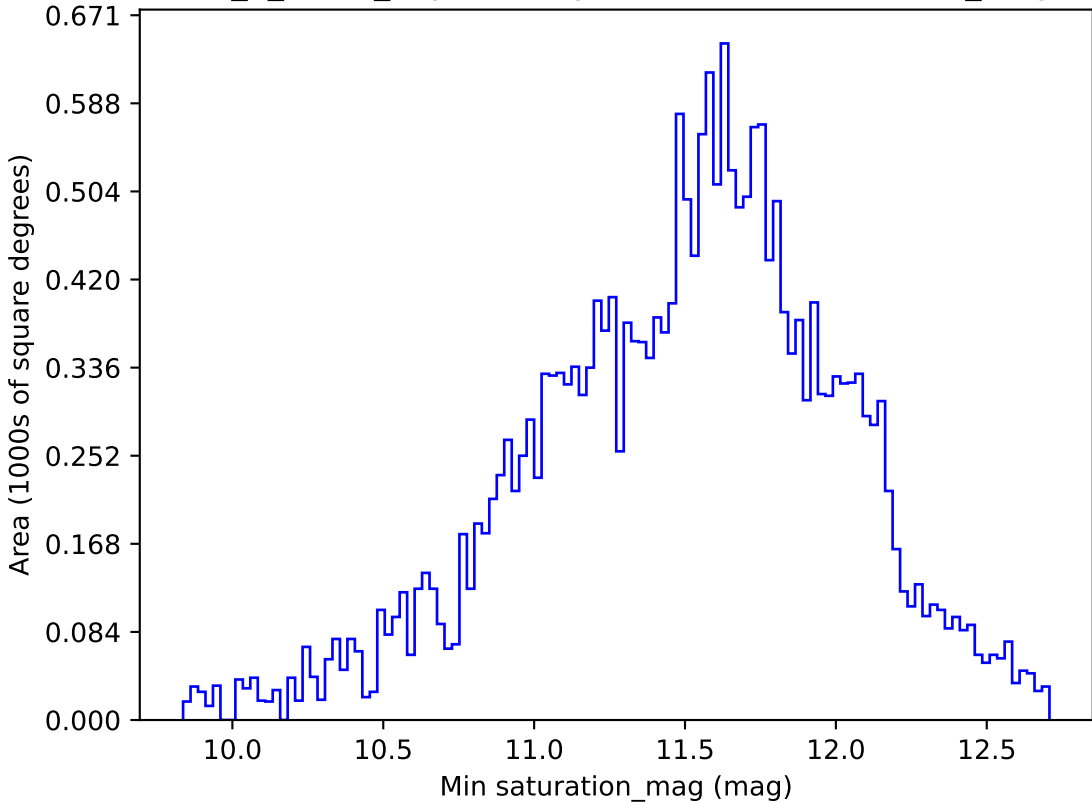
too_5_1v3.4_10yrs All sky u band: Min saturation_mag
