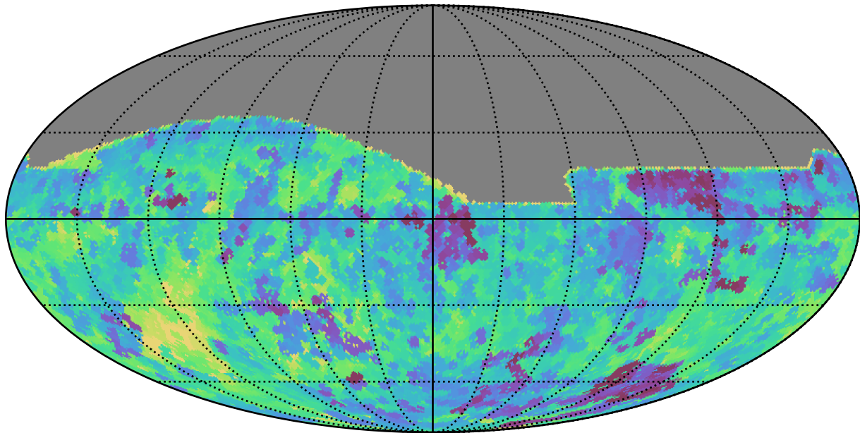
too_5_1v3.4_10yrs All sky r band: Min saturation_mag
