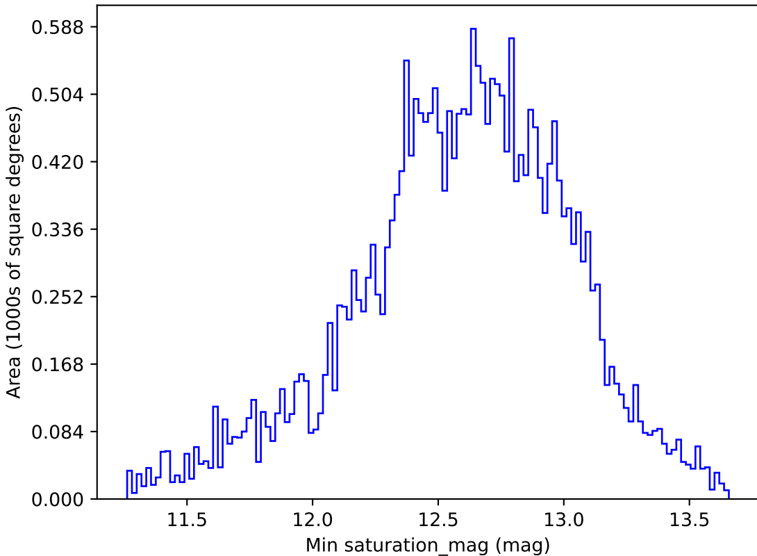
too_5_1v3.4_10yrs All sky r band: Min saturation_mag
