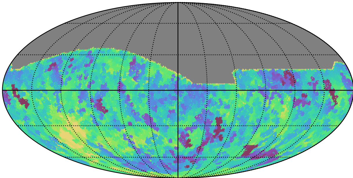
too_5_1v3.4_10yrs All sky i band: Min saturation_mag
